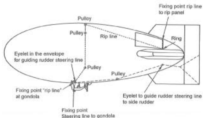
Figure 23.9. The AS 105 GD four-scater hot air airship.
